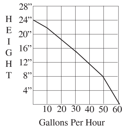
FT-40 FLOW CHART
